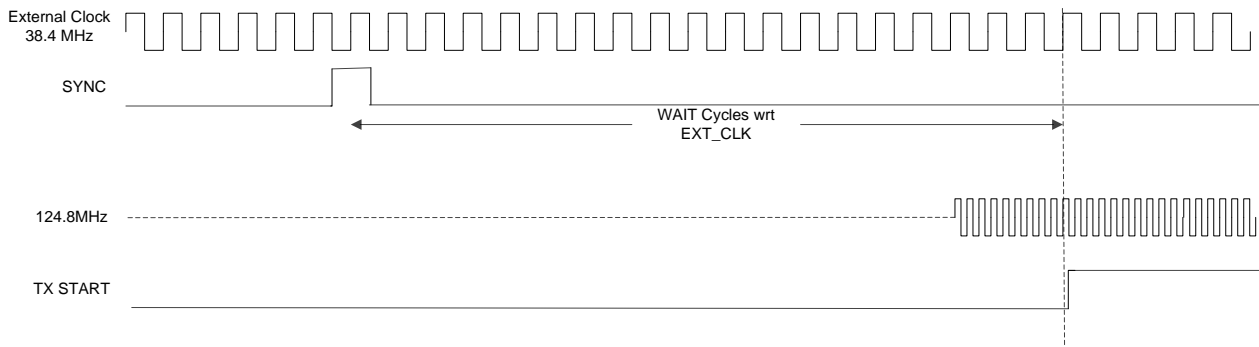
Figure 24: Synchronised Transmission
